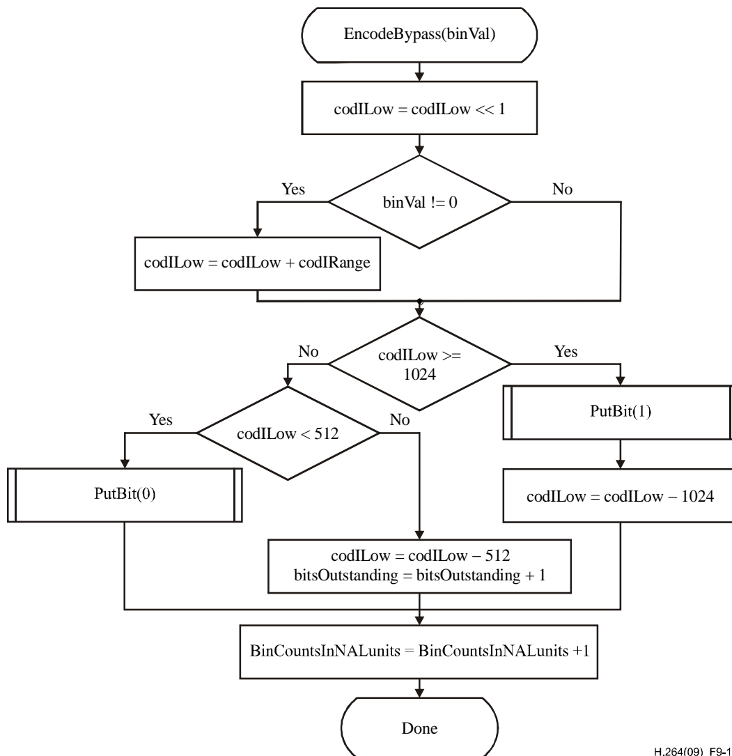
Figure 9-10 – Flowchart of encoding bypass
