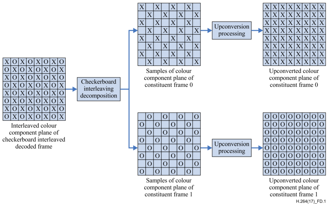
Figure D-1 – Rearrangement and upconversion of checkerboard interleaving (frame_packing_arrangement_type equal to 0)
