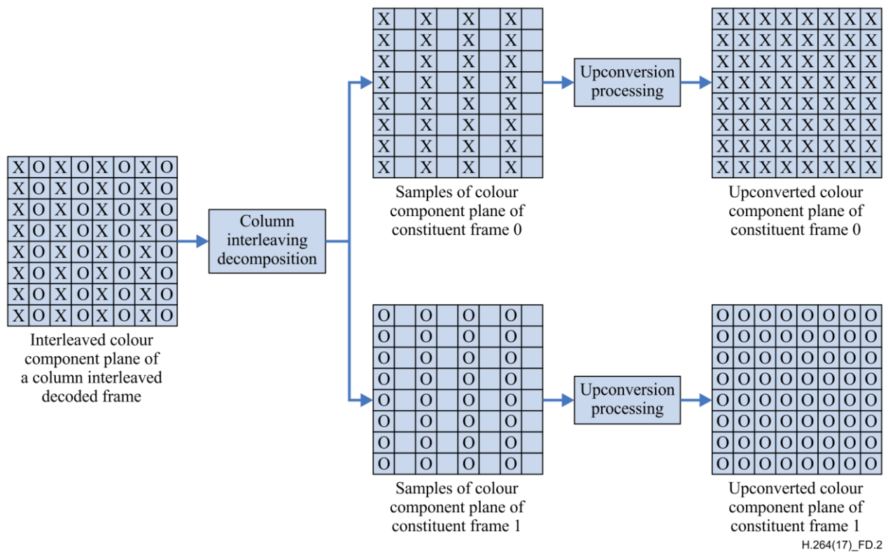
Figure D-2 – Rearrangement and upconversion of column interleaving with frame_packing_arrangement_type equal to 1, quincunx_sampling_flag equal to 0, and (x, y) equal to (0, 0) or (4, 8) for both constituent frames
