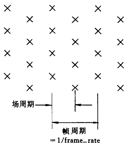
图 I -7-20 progressive_sequence == 0
