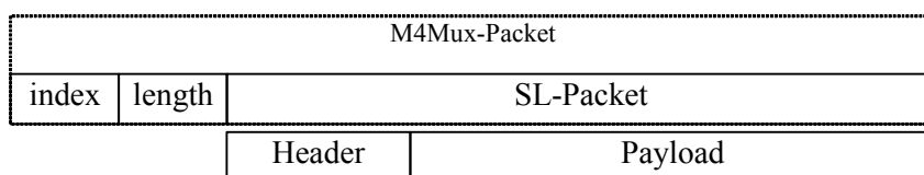
Figure 11 — Structure of M4Mux packet in simple mode
