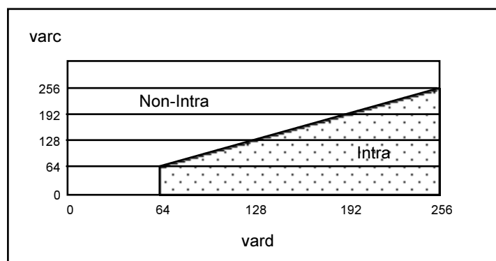
Figure 2-D.34 Characteristic Intra/Non-Intra
