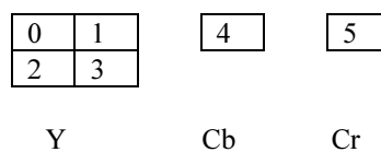
Figure 2-2 The arrangement of blocks in a macroblock.
