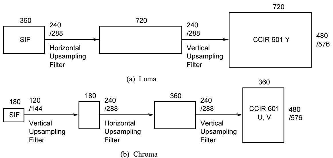
Figure 2-D.41 Simplified Decoder Block Diagram
