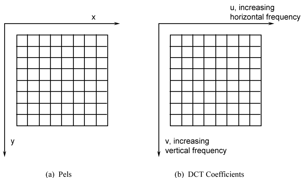
Figure 2-D.28 Transformation of Pixels to Coefficients
