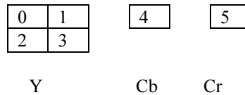
Figure 2-D.5 Macroblock Structure
