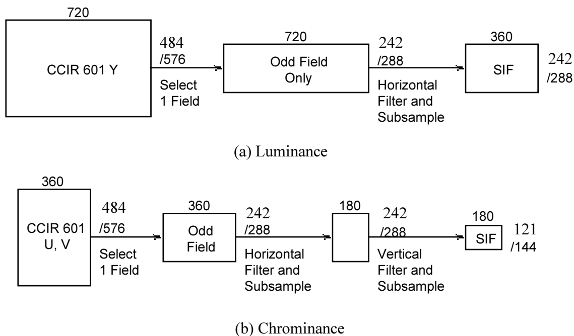
Figure 2-D.12 Conversion from CCIR 601 into SIF
