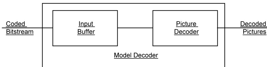
Figure 2-D.14 Model Decoder
