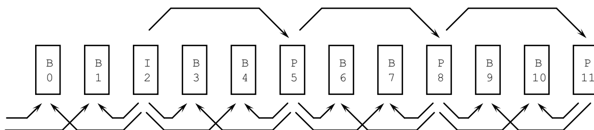
Figure 2-D.2 Dependency Relationship Between I, B, and P-pictures
