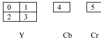
Figure 2-I.3 Macroblock Structure
